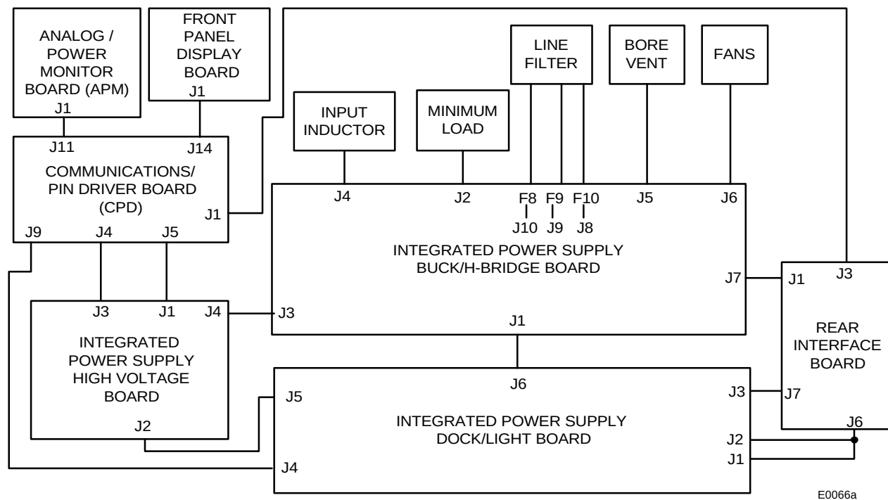
SYSTEM SUPPORT MODULE INTERCONNECTS ILLUSTRATION 2-3
