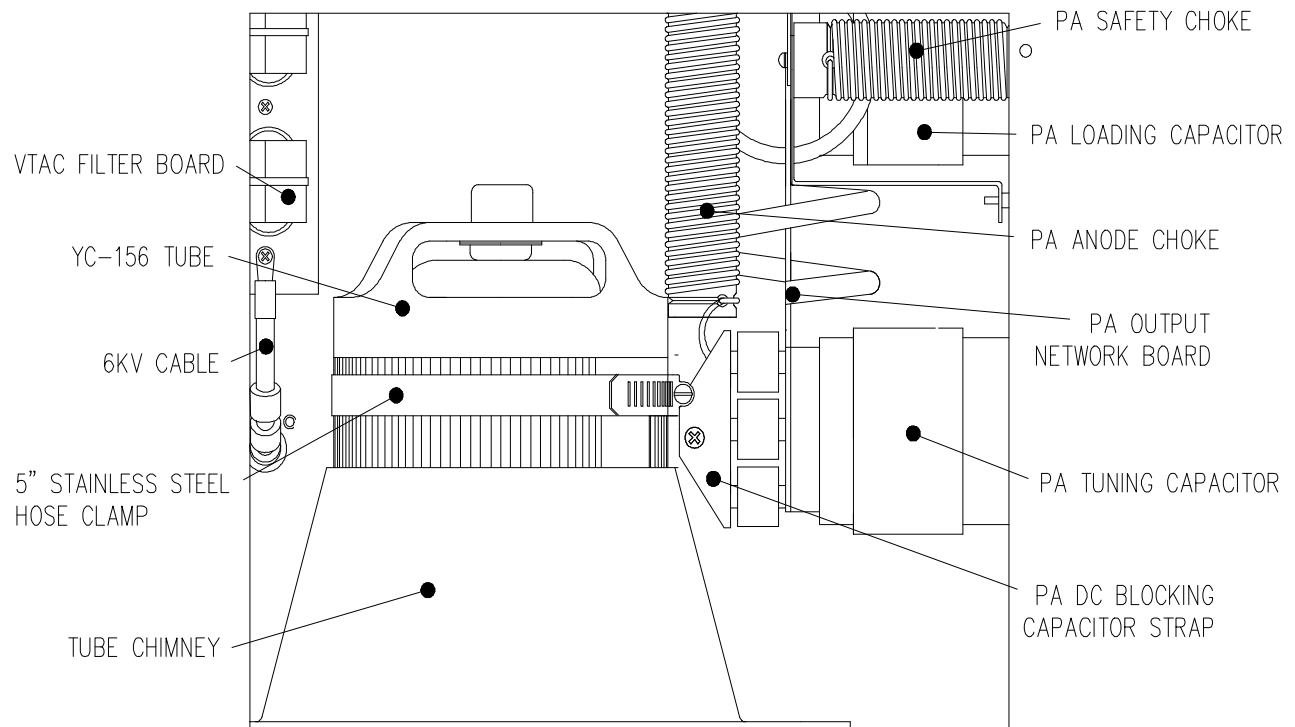
RF AMPLIFIER (1.0T) COMPONENT LOCATIONS/PA CAVITY DETAIL ILLUSTRATION 1-11
