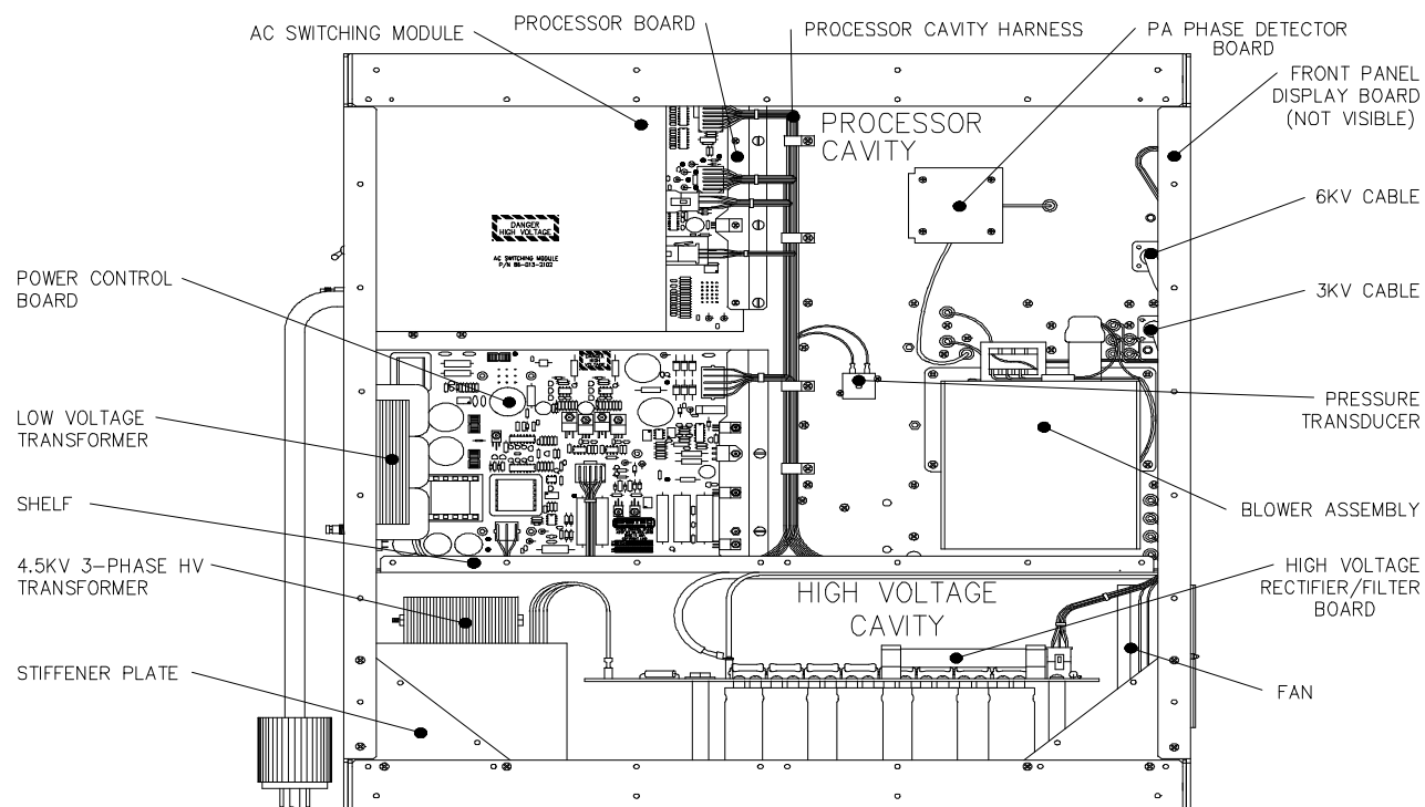
RF AMPLIFIER (1.5T) COMPONENT LOCATIONS/PROCESSOR AND HIGH VOLTAGE CAVITIES ILLUSTRATION 1-5
