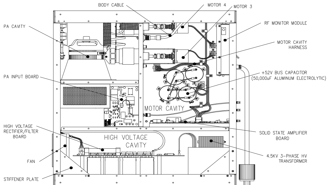
RF AMPLIFIER (1.0T) COMPONENT LOCATION/MOTOR, HIGH VOLTAGE, AND PA CAVITIES ILLUSTRATION 1-10
