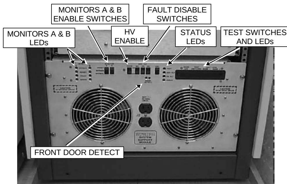
FRONT SSM LOCATIONS DETAIL ILLUSTRATION 1-2
