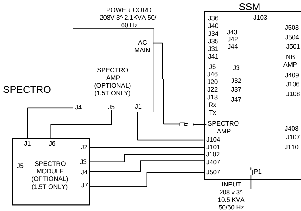
RF/PEN II CABINET INTERCONNECTS - SPECTROSCOPY OPTION ILLUSTRATION 2-2
