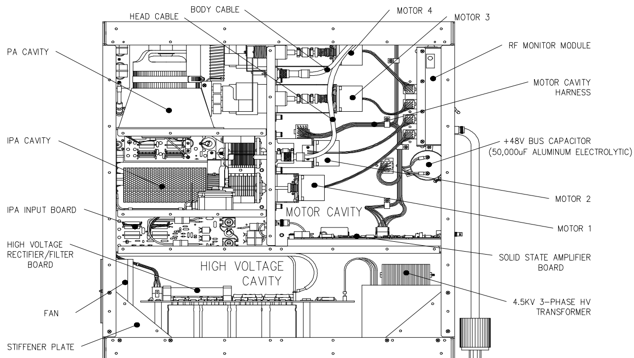
RF AMPLIFIER (1.5T) COMPONENT LOCATIONS/MOTOR, HIGH VOLTAGE, PA, AND IPA (VTAC) ILLUSTRATION 1-6
