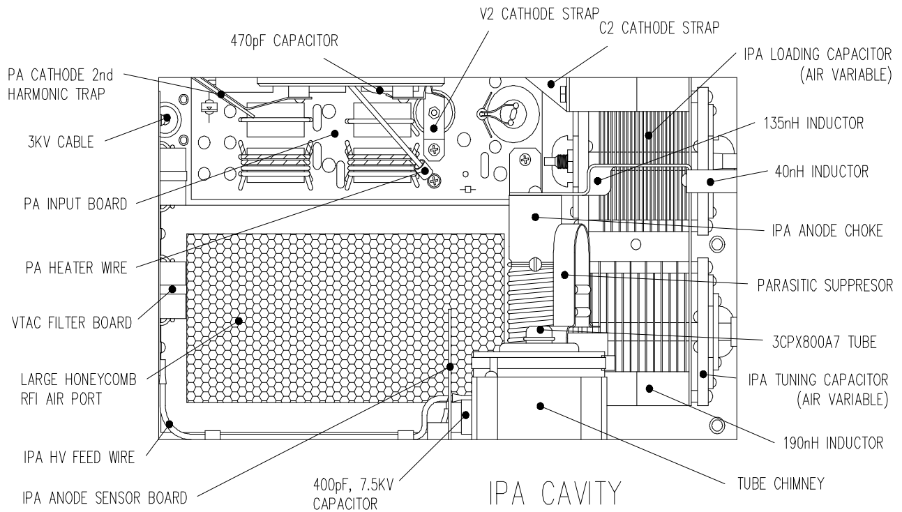
RF AMPLIFIER (1.5T) COMPONENT LOCATIONS/IPA CAVITY DETAIL ILLUSTRATION 1-8
