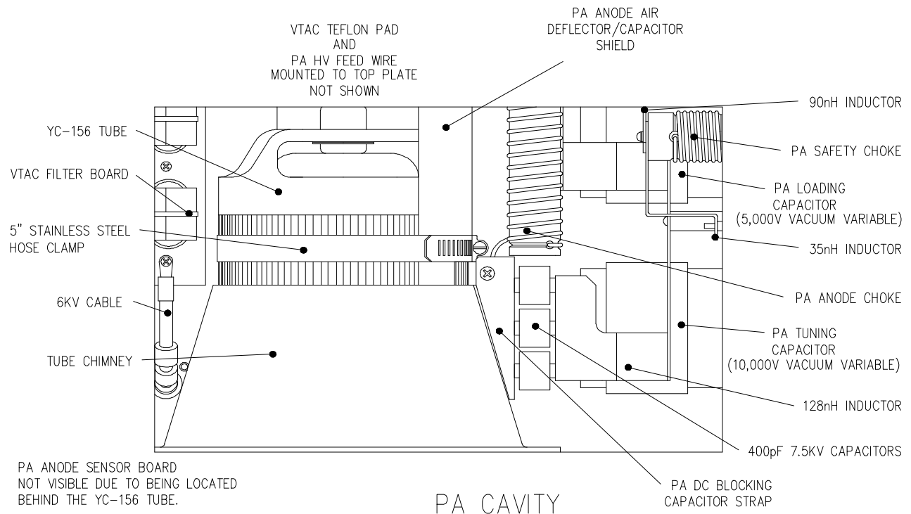
RF AMPLIFIER (1.5T) COMPONENT LOCATIONS/PA CAVITY DETAIL ILLUSTRATION 1-7
