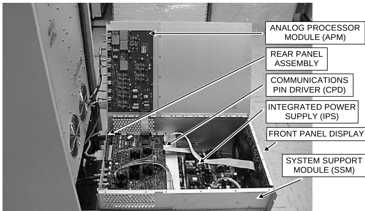
SSM COMPONENT LOCATIONS ILLUSTRATION 1-1
