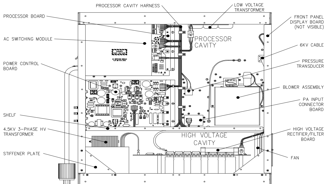
RF AMPLIFIER (1.0T) COMPONENT LOCATIONS/PROCESSOR AND HIGH VOLTAGE CAVITIES ILLUSTRATION 1-9
