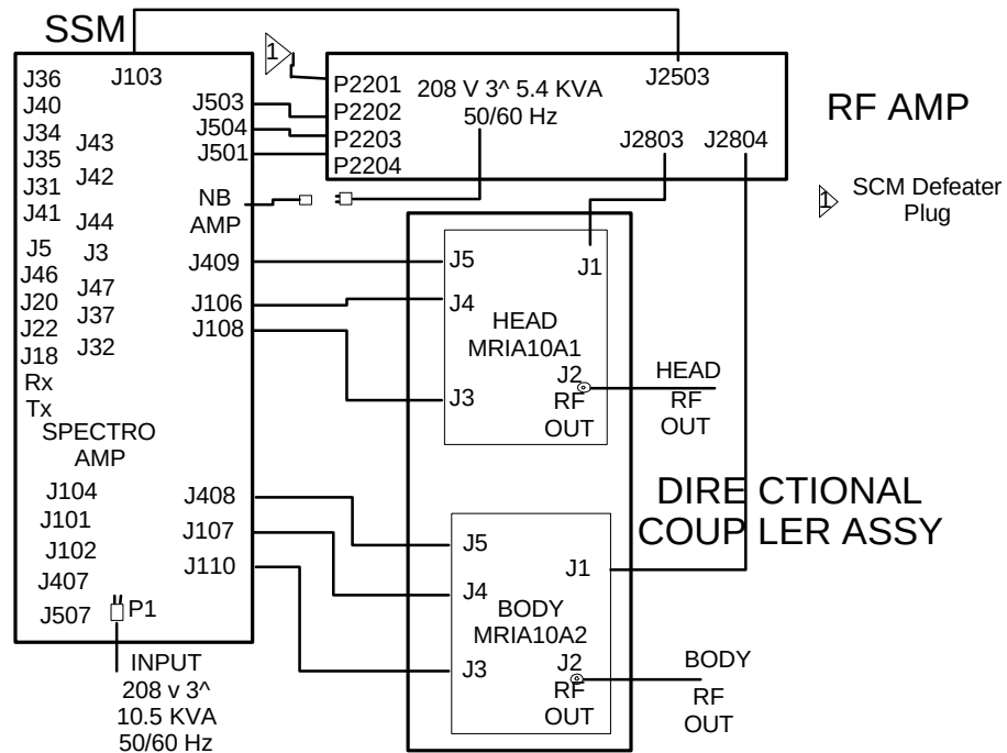
RF/PEN II CABINET INTERCONNECTS ILLUSTRATION 2-1
